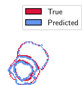
segmentations
